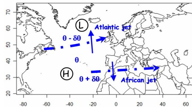
Fig. 4. Conceptual picture of the vorticity and thermal advections driven by the cross-jet circulations in the exit region of the Atlantic jet and in the entrance region of the African jet.
