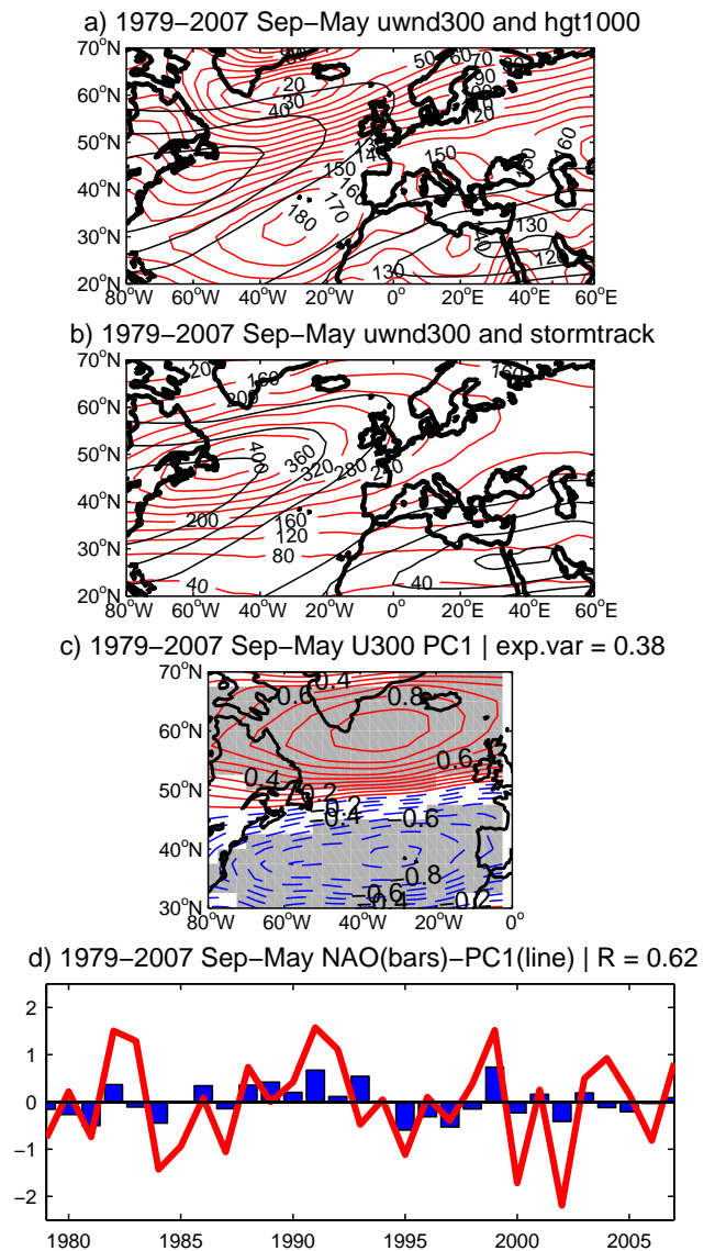
Fig. 1. September to May climatology: (a) geopotential at 1000 hPa (m) (red contours); (b) stormtrack at 300 hPa ( m^2 s^{-2} ) (red contours); (a) and (b) the zonal wind at 300 hPa (black contours, 5 m s^{-1} interval beginning at 15 m s^{-1} ). September to May interannual variability: (c) 1st PC of the 300 hPa zonal wind (PC1) in homogeneous correlation maps (positive values in red, negative values dashed in blue, 95 % significance shaded in gray); (d) PC1 time-series (red line) and NAO index (blue bars).
