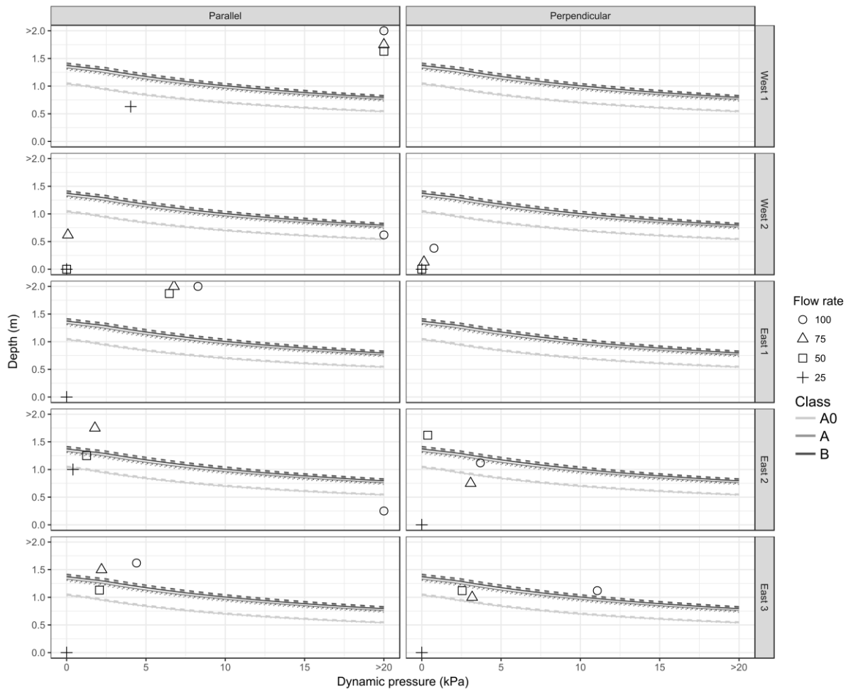
Figure S3. Critical depth-pressure curves for building classes A0, A and B with brick widths of 0.25 m subjected to a debris flow. Peak normal pressures and corresponding depths applied to each city block are plotted as points for each flow rate.
