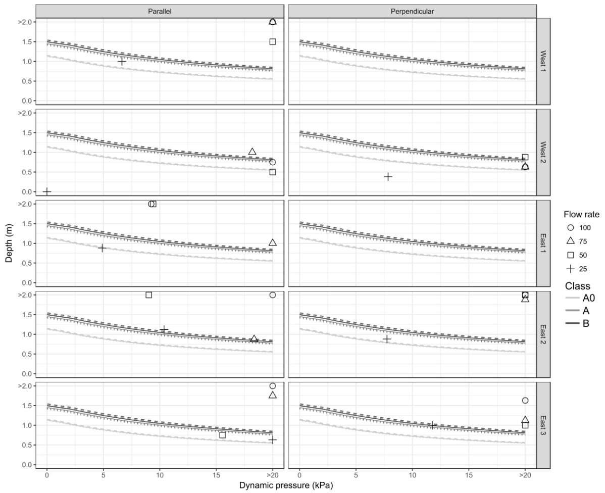
Figure S2. Critical depth-pressure curves for building classes A0, A and B with brick widths of 0.25 m subjected to a hyperconcentrated flow. Peak normal pressures and corresponding depths applied to each city block are plotted as points for each flow rate.
