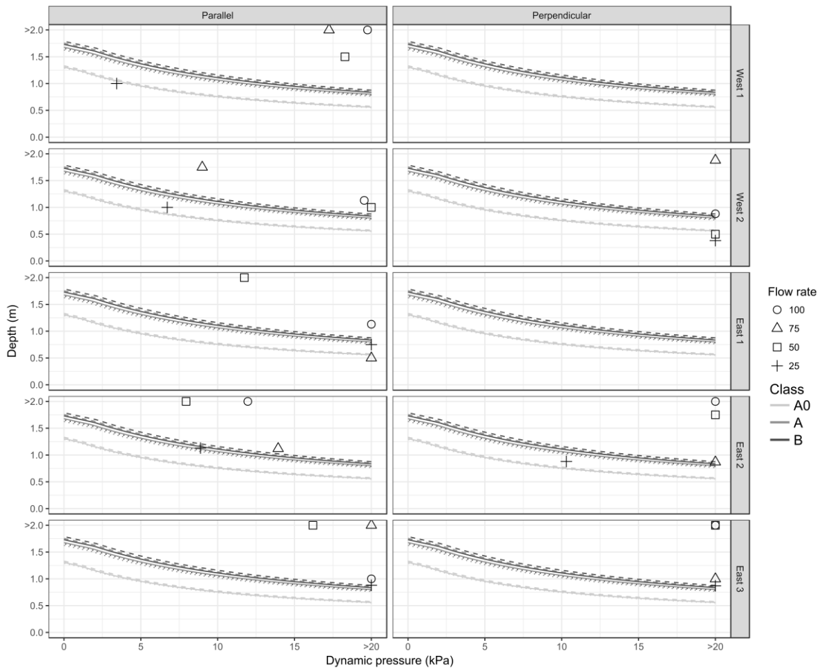
Figure S1. Critical depth-pressure curves for building classes A0, A and B with brick widths of 0.25 m subjected to Newtonian flow. Peak normal pressures and corresponding depths applied to each city block are plotted as points for each flow rate.
