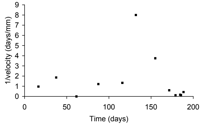
Fig. 6. Displacements of the landslide surface for Inclinator 10, plotted in \Lambda-t space.
