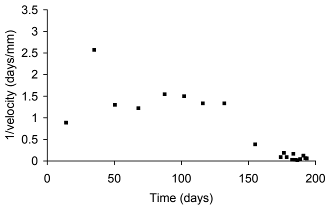
Fig. 5. Displacements of the landslide surface for Inclinator 9, plotted in \Lambda-t space.
