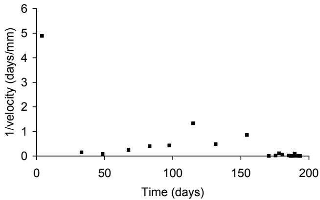
Fig. 4. Displacements of the landslide surface for Inclinator 4, plotted in \Lambda-t space.
